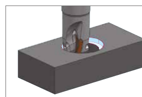
Hole expansion milling
