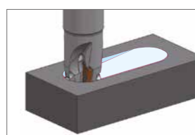
Ramping
