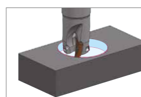
Helical milling
